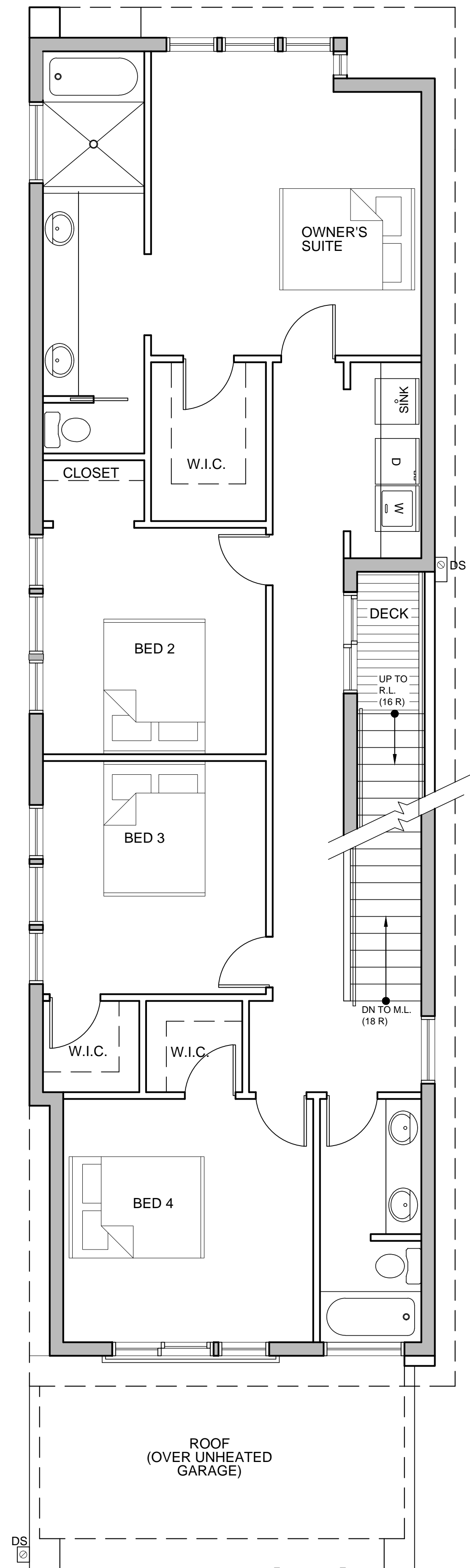
UPPER LEVEL F.F. 264.6' SCALE: 1/4" = 1'-0" 1279 SF + 23 SF DECK
