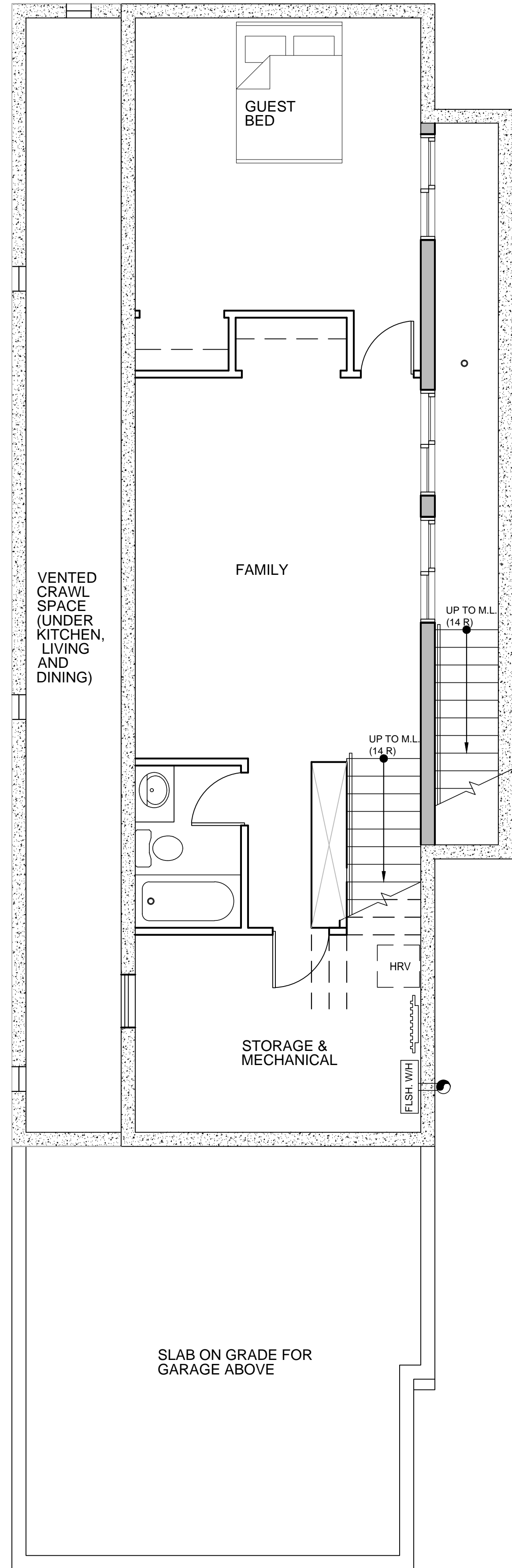
LOWER LEVEL F.F. 245.1' SCALE: 1/4" = 1'-0" 800 SF
